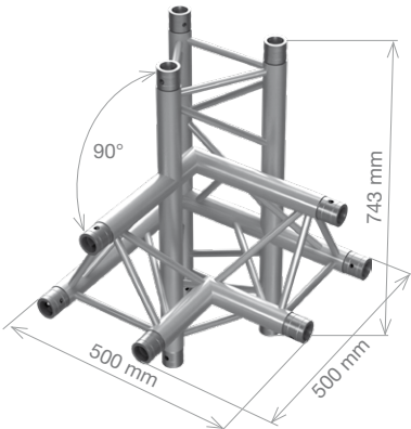
PT33-C44 PTH33-C44 4-way 90° right corner 0.74 x 0.5 x 0.5 m (2.44 x 1.64 x 1.64 ft) 7.33 kg (16.16 lbs) 8.37 kg (18.45 lbs)
