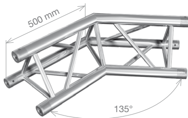
FT33-C23 HT33-C23 2-way 135° corner 0.5 m (1.64 ft) 4.1 kg (9.09 lbs) 4.7 kg (10.30 lbs)
