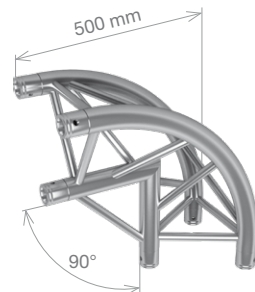
FT33-C25-R 2-way 90° rounded corner, apex in 0.5 m (1.64 ft) 3.5 kg (7.79 lbs)
