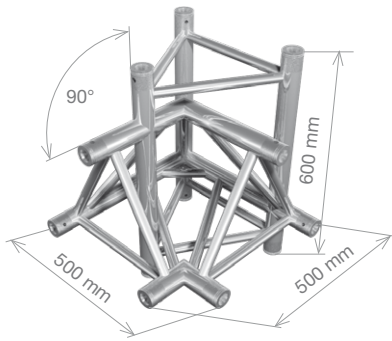
FT43-C44 HT43-C44 4-way 90° right corner 0.5 m (1.64 ft) 8.05 kg (17.75 lbs) 9.04 kg (19.92 lbs)
