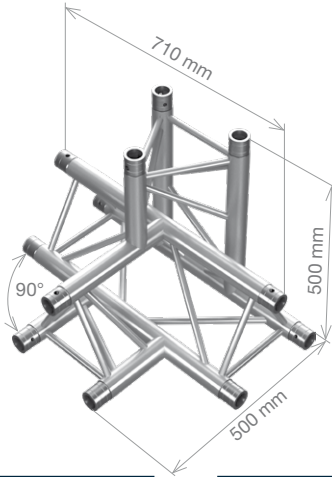
PT33-T42 PTH33-T42 4-way T-junction, apex down 0.71 x 0.5 x 0.5 m (2.33 x 1.64 x 1.64 ft) 6.98 kg (15.38 lbs) 8.57 kg (18.89 lbs)
