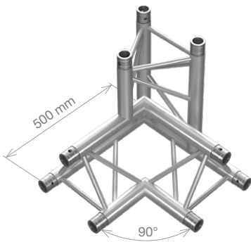
PT33-C34 PTH33-C34 3-way 90° left corner, apex down 0.5 m (1.64 ft) 5.67 kg (12.51 lbs) 6.99 kg (15.42 lbs)
