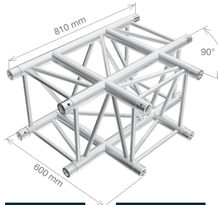
PT44-T35 PTH44-T35 3-way T-junction 0.81 x 0.6 m (2.66 x 1.97 ft) 9.59 kg (21.14 lbs) 11.60 kg (25.57 lbs)
