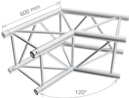
PT44-C22 PTH44-C22 2-way 120° corner 0.6 m (1.97 ft) 6.92 kg (15.26 lbs) 12.36 kg (27.15 lbs)
