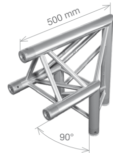
FT33-C24 HT33-C24 2-way 90° corner, apex out 0.5 m (1.64 ft) 3.7 kg (8.16 lbs) 4.3 kg (9.57 lbs)
