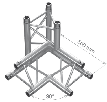
PT33-C33 PTH33-C33 3-way 90° right corner, apex down 0.5 m (1.64 ft) 5.67 kg (12.51 lbs) 6.99 kg (15.42 lbs)
