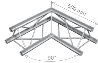
FT23-C21 2-way 90° corner, apex up / down 0.5 m (1.64 ft) 2.2 kg (4.82 lbs)
