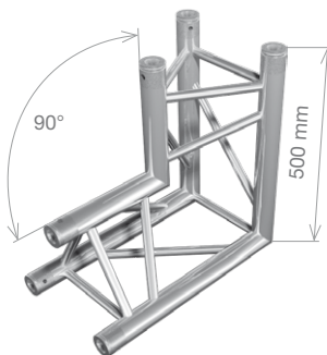
FT33-C25 HT33-C25 2-way 90° corner, apex in 0.5 m (1.64 ft) 3.9 kg (8.58 lbs) 4.7 kg (10.39 lbs)
