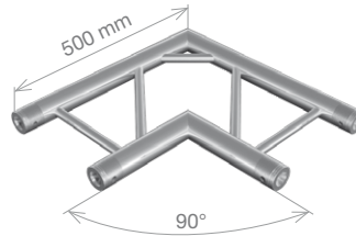
FT32-C21H HT32-C21H 2-way 90° horizontal corner 0.5 m (1.64 ft) 2.2 kg (4.78 lbs) 2.6 kg (5.67 lbs)
