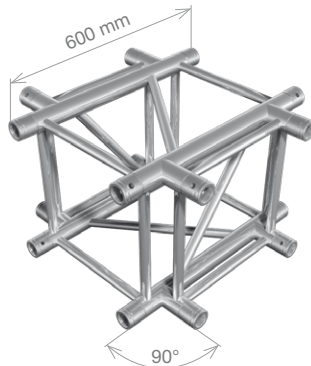
FT44-C41 HT44-C41 4-way cross junction 0.6 m (1.97 ft) 8.56 kg (18.85 lbs) 9.35 kg (20.62 lbs)
