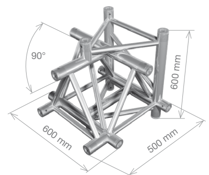
FT43-T51 HT43-T51 5-way T-junction, apex down 0.6 x 0.6 x 0.5 m (1.97 x 1.97 x 1.64 ft) 8.33 kg (18.35 lbs) 9.30 kg (20.49 lbs)
