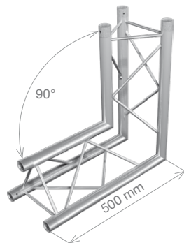
FT23-C25 2-way 90° corner, apex in 0.5 m (1.64 ft) 2.3 kg (4.99 lbs)
