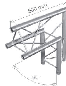
FT23-C24 2-way 90° corner, apex out 0.5 m (1.64 ft) 2.0 kg (4.32 lbs)
