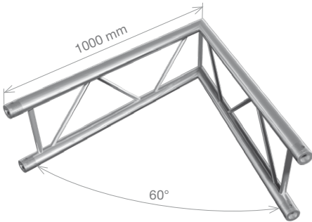
FT32-C20V HT32-C20V 2-way 60° vertical corner 1 m (3.28 ft) 4.6 kg (10.07 lbs) 6.0 kg (13.18 lbs)
