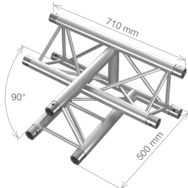
PT33-T35 PTH33-T35 3-way vertical T-junction, apex down 0.71 x 0.5 m (2.33 x 1.64 ft) 5.82 kg (12.82 lbs) 7.23 kg (15.93 lbs)
