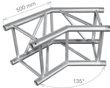
FT44-C23 HT44-C23 2-way 135° corner 0.5 m (1.64 ft) 6.93 kg (15.28 lbs) 7.33 kg (16.16 lbs)
