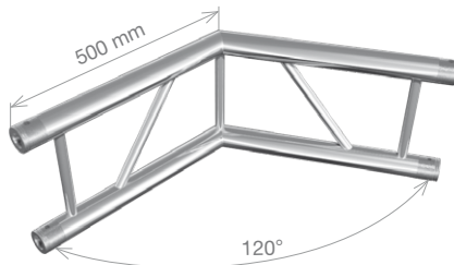
FT32-C22V HT32-C22V 2-way 120° vertical corner 0.5 m (1.64 ft) 2.6 kg (5.67 lbs) 2.5 kg (5.49 lbs)
