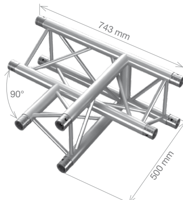
PT33-T38 PTH33-T38 3-way vertical T-junction, apex down 0.74 x 0.5 m (2.44 x 1.64 ft) 5.73 kg (12.63 lbs) 7.10 kg (15.66 lbs)
