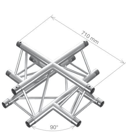
PT33-C41 PTH33-C41 4-way cross junction 0.71 x 0.71 m (2.33 x 2.33 ft) 6.58 kg (14.50 lbs) 8.04 kg (17.72 lbs)
