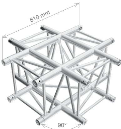
PT44-C41 PTH44-C41 4-way cross junction 0.81 m (2.66 ft) 11.86 kg (26.15 lbs) 14.26 kg (31.43 lbs)
