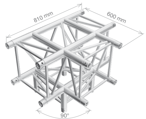
PT44-T42 PTH44-T42 4-way T-junction 0.81 x 0.6 m (2.66 x 1.97 ft) 11.84 kg (26.11 lbs) 14.25 kg (31.42 lbs)
