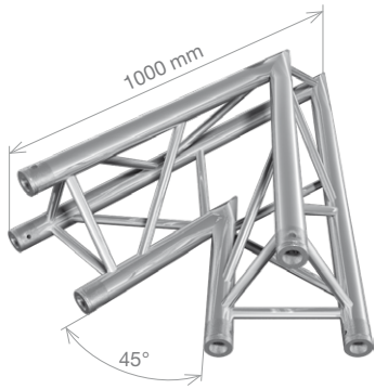
FT33-C19 HT33-C19 2-way 45° corner 1 m (3.28 ft) 5.7 kg (12.56 lbs) 7.2 kg (15.77 lbs)
