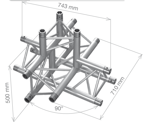
PT33-T51 PTH33-T51 5-way T-junction, apex down 0.74 x 0.71 x 0.5 m (2.44 x 2.33 x 1.64 ft) 8.64 kg (19.04 lbs) 9.99 kg (22.03 lbs)
