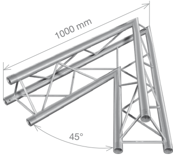
FT23-C19 2-way 45° corner 1 m (3.28 ft) 3.8 kg (8.39 lbs)
