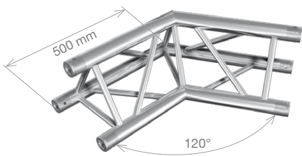
FT33-C22 HT33-C22 2-way 120° corner 0.5 m (1.64 ft) 4.1 kg (9.09 lbs) 4.5 kg (10.00 lbs)
