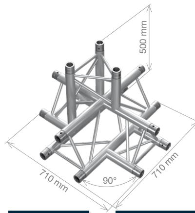
PT33-C53 PTH33-C53 5-way cross junction, apex down 0.71 x 0.71 x 0.5 m (2.33 x 2.33 x 1.64 ft) 8.48 kg (18.70 lbs) 10.39 kg (22.90 lbs)
