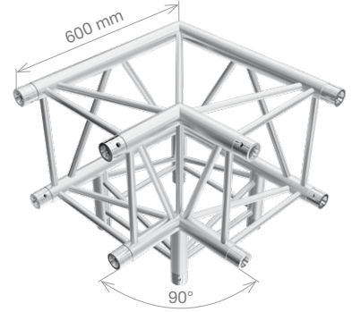
PT44-C30 PTH44-C30 3-way 90° corner 0.6 m (1.97 ft) 8.73 kg (19.25 lbs) 10.41 kg (22.96 lbs)
