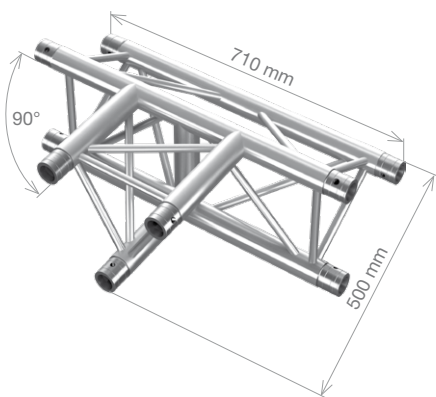
PT33-T37 PTH33-T37 3-way horizontal T-junction, apex up 0.71 x 0.5 m (2.33 x 1.64 ft) 5.25 kg (11.57 lbs) 6.45 kg (14.23 lbs)
