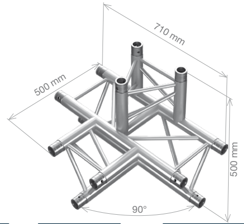
PT33-T43 PTH33-T43 4-way T-junction, apex up 0.71 x 0.5 x 0.5 m (2.33 x 1.64 x 1.64 ft) 6.73 kg (14.84 lbs) 8.26 kg (18.20 lbs)
