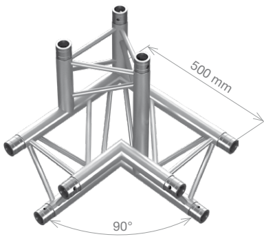
PT33-C31 PTH33-C31 3-way 90° right corner, apex up 0.5 m (1.64 ft) 5.43 kg (11.96 lbs) 6.68 kg (14.72 lbs)
