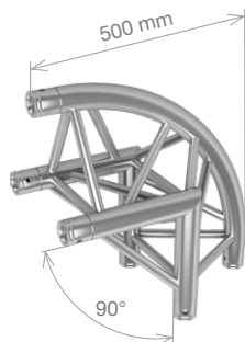
FT33-C24-R 2-way 90° rounded corner, apex out 0.5 m (1.64 ft) 3.5 kg (7.79 lbs)
