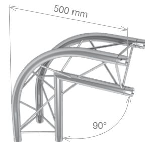
FT23-C25-R 2-way 90° rounded corner, apex in 0.5 m (1.64 ft) 2.3 kg (4.99 lbs)
