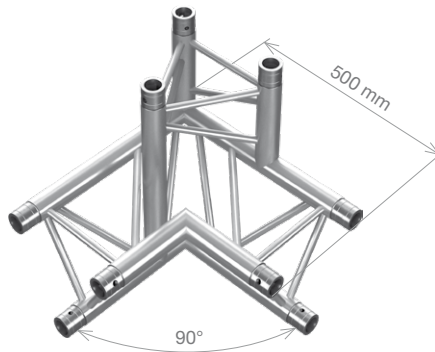
PT33-C32 PTH33-C32 3-way 90° left corner, apex up 0.5 m (1.64 ft) 5.43 kg (11.96 lbs) 6.68 kg (14.72 lbs)
