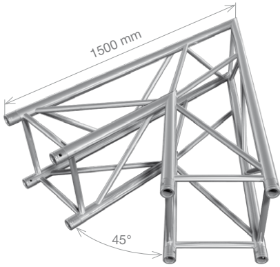
FT44-C19 HT44-C19 2-way 45° corner 1.5 m (4.92 ft) 14.09 kg (31.07 lbs) 17.15 kg (37.81 lbs)
