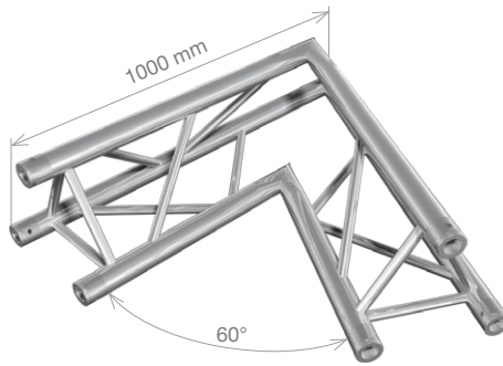
FT33-C20 HT33-C20 2-way 60° corner 1 m (3.28 ft) 6.1 kg (13.42 lbs) 7.7 kg (17.04 lbs)
