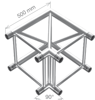
FT44-C21 HT44-C21 2-way 90° corner 0.5 m (1.64 ft) 6.08 kg (13.41 lbs) 6.70 kg (14.78 lbs)
