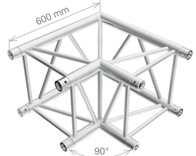
PT44-C21 PTH44-C21 2-way 90° corner 0.6 m (1.97 ft) 6.50 kg (14.34 lbs) 7.81 kg (17.23 lbs)
