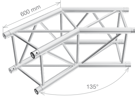
PT44-C23 PTH44-C23 2-way 135° corner 0.6 m (1.97 ft) 7.31 kg (16.12 lbs) 8.87 kg (19.56 lbs)
