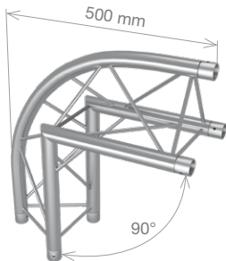
FT23-C24-R 2-way 90° rounded corner, apex out 0.5 m (1.64 ft) 2.0 kg (4.32 lbs)
