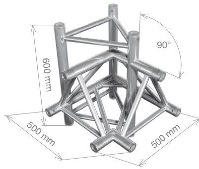
FT43-C45 HT43-C45 4-way 90° left corner 0.5 m (1.64 ft) 8.05 kg (17.75 lbs) 9.04 kg (19.92 lbs)
