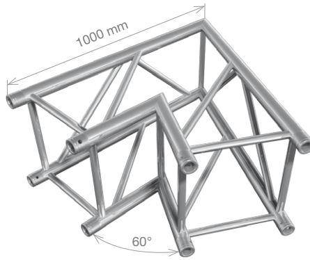
FT44-C20 HT44-C20 2-way 60° corner 1 m (3.28 ft) 9.50 kg (20.94 lbs) 11.40 kg (25.13 lbs)
