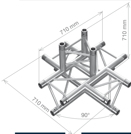
PT33-C52 PTH33-C52 5-way cross junction, apex up 0.71 x 0.71 x 0.5 m (2.33 x 2.33 x 1.64 ft) 8.23 kg (18.15 lbs) 10.08 kg (22.22 lbs)
