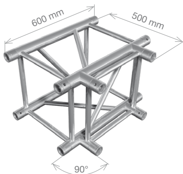
FT44-T35 HT44-T35 3-way T-junction 0.6 x 0.5 m (1.97 x 1.64 ft) 6.94 kg (15.30 lbs) 7.69 kg (16.95 lbs)
