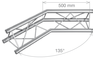
FT23-C23 2-way 135° corner 0.5 m (1.64 ft) 2.5 kg (5.49 lbs)
