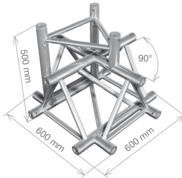
FT43-C53 HT43-C53 5-way cross junction, apex down 0.6 x 0.6 x 0.5 m (1.97 x 1.97 x 1.64 ft) 8.74 kg (19.26 lbs) 9.80 kg (21.60 lbs)
