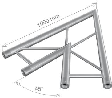
FT32-C19H HT32-C19H 2-way 45° horizontal corner 1 m (3.28 ft) 4.0 kg (8.79 lbs) 5.2 kg (11.56 lbs)
