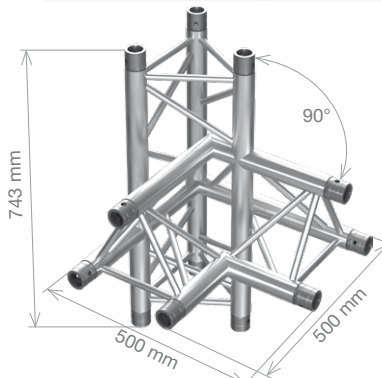
PT33-C45 PTH33-C45 4-way 90° left corner 0.74 x 0.5 x 0.5 m (2.44 x 1.64 x 1.64 ft) 7.33 kg (16.16 lbs) 8.37 kg (18.45 lbs)
