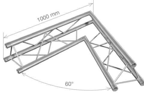
FT23-C20 2-way 60° corner 1 m (3.28 ft) 4.2 kg (9.29 lbs)
