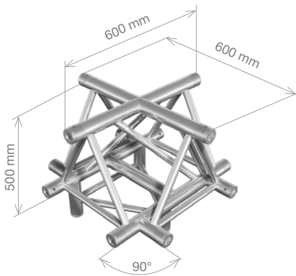
FT43-C52 HT43-C52 5-way cross junction, apex up 0.6 x 0.6 x 0.5 m (1.97 x 1.97 x 1.64 ft) 7.92 kg (17.47 lbs) 8.64 kg (19.05 lbs)
