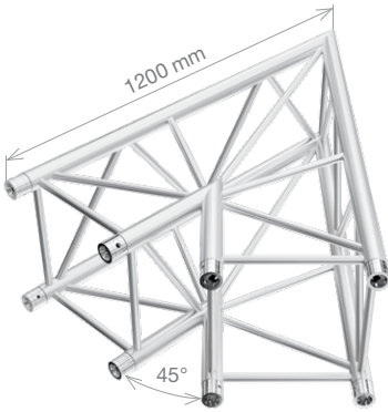
PT44-C19 PTH44-C19 2-way 45° corner 1.2 m (3.94 ft) 10.06 kg (22.18 lbs) 12.36 kg (27.15 lbs)
