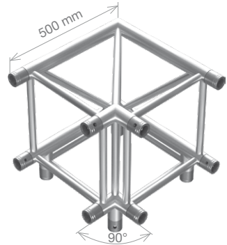
FT44-C30 HT44-C30 3-way 90° corner 0.5 m (1.64 ft) 7.70 kg (16.98 lbs) 8.38 kg (18.47 lbs)
