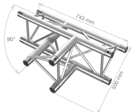
PT33-T39 PTH33-T39 3-way vertical T-junction 0.74 x 0.5 m (2.44 x 1.64 ft) 5.33 kg (11.74 lbs) 6.56 kg (14.47 lbs)
