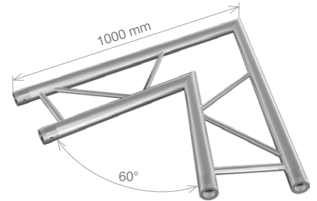
FT32-C20H HT32-C20H 2-way 60° horizontal corner 1 m (3.28 ft) 3.7 kg (8.26 lbs) 4.8 kg (10.68 lbs)
