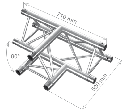
PT33-T36 PTH33-T36 3-way horizontal T-junction 0.71 x 0.5 m (2.33 x 1.64 ft) 5.07 kg (11.18 lbs) 6.22 kg (13.70 lbs)
