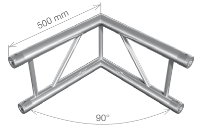
FT32-C21V HT32-C21V 2-way 90° vertical corner 0.5 m (1.64 ft) 2.6 kg (5.67 lbs) 3.2 kg (7.11 lbs)
