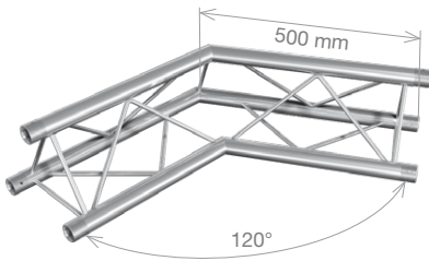
FT23-C22 2-way 120° corner 0.5 m (1.64 ft) 2.4 kg (5.38 lbs)
