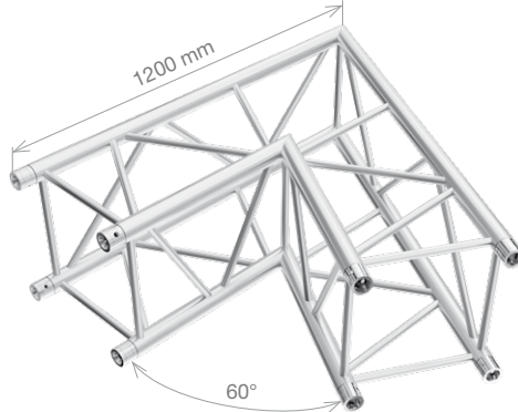
PT44-C20 PTH44-C20 2-way 60° corner 1.2 m (3.94 ft) 10.87 kg (22.96 lbs) 13.43 kg (29.61 lbs)
