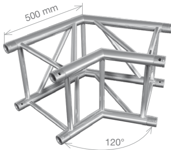
FT44-C22 HT44-C22 2-way 120° corner 0.5 m (1.64 ft) 6.74 kg (14.87 lbs) 6.68 kg (14.73 lbs)
