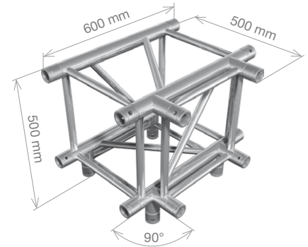
FT44-T42 HT44-T42 4-way T-junction 0.6 x 0.5 x 0.5 m (1.97 x 1.64 x 1.64 ft) 8.56 kg (18.85 lbs) 9.35 kg (20.62 lbs)
